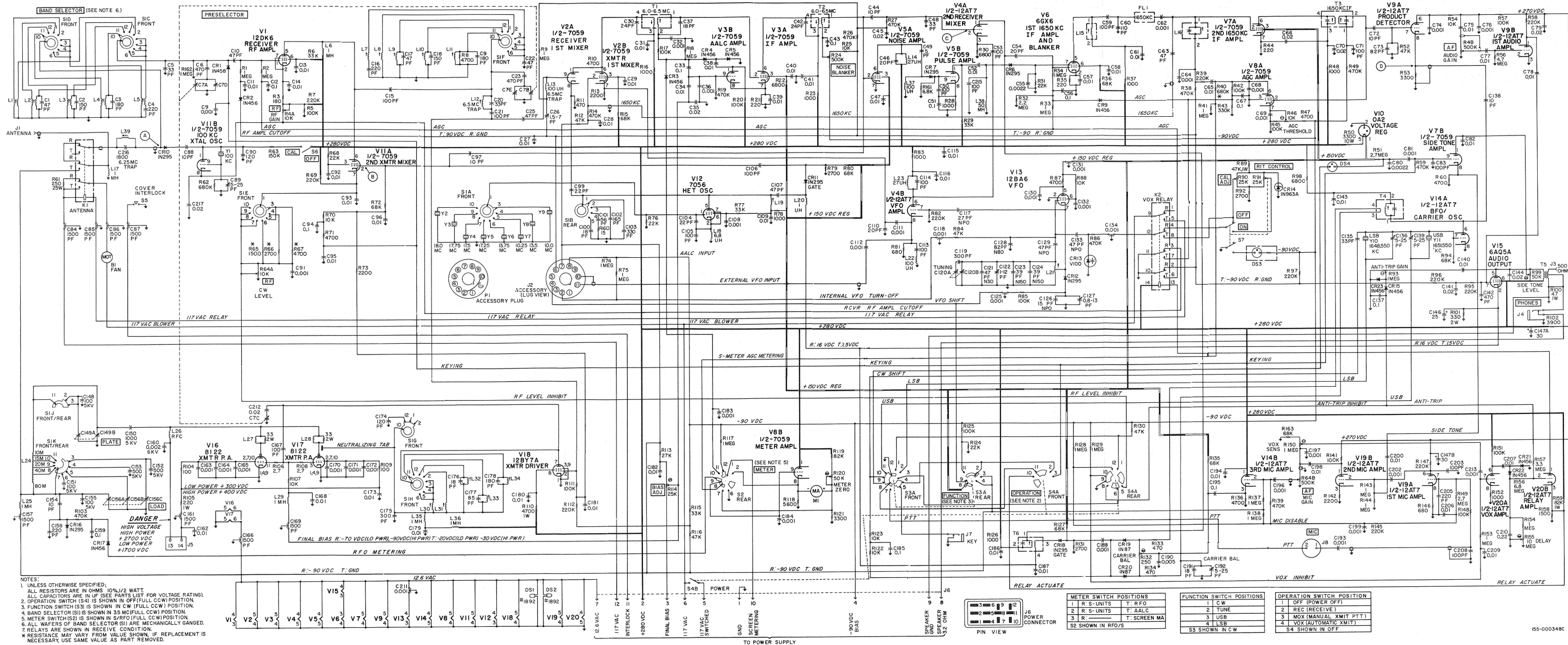
Figure 22. Model SR-2000 Transceiver Schematic Diagram.
